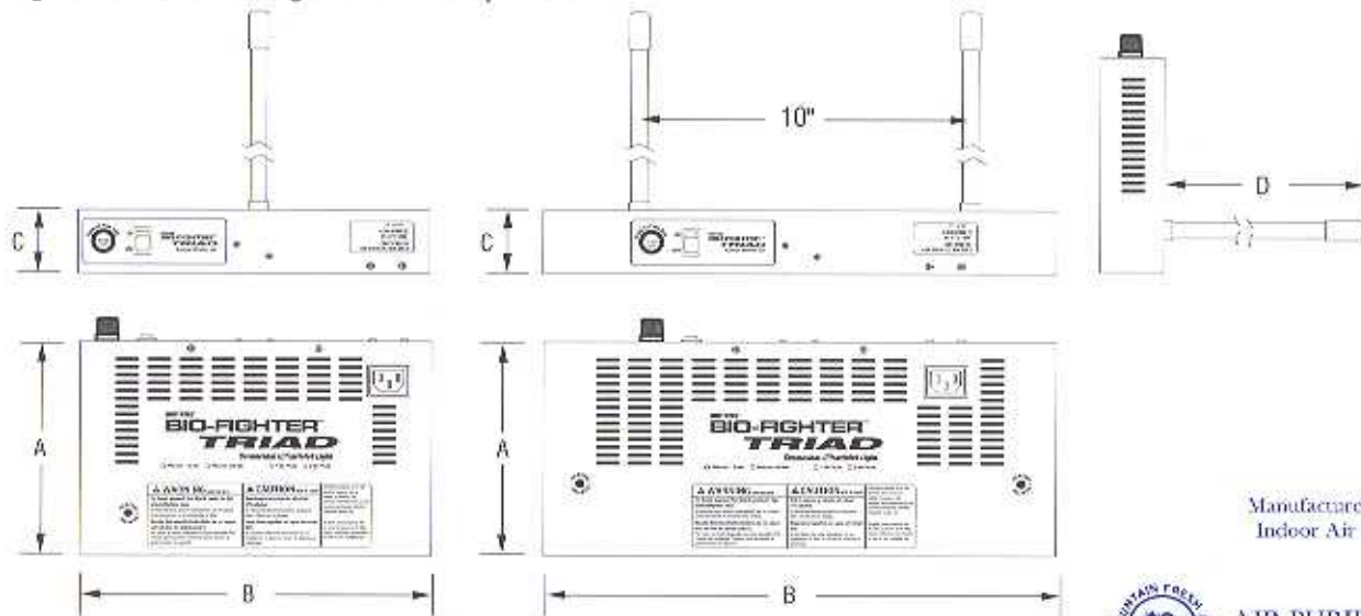
Fig. 3 Dimensions of single and dual lamp Triads.
